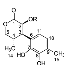
O -Acetylcalopin ( 1a ), R = Ac Calopin ( 1b ), R = H
