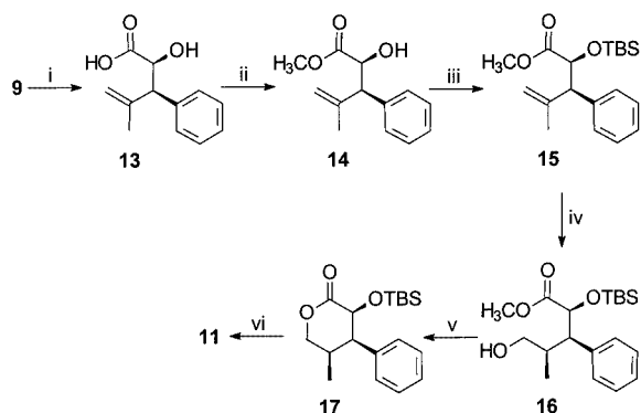
Scheme 3. Alternative synthesis of all- cis - \delta -valerolactone 11 ; reagents and conditions: i) NaOH, THF, MeOH, \Delta (90%); ii) SOCl 2 , MeOH, cat. DMF, \Delta (79%); iii) TBSOTf, 2,6-lutidine, DMAP, CH 2 Cl 2 (85%); iv) 9-BBN, THF, then NaOH, H 2 O 2 , ultra sound (98%); v) TFA, CHCl 3 (96%); vi) concd. HCl, THF, MeOH (42%); TFA = trifluoroacetic acid (concd. = concentrated)
