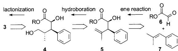
Scheme 1. Retrosynthetic analysis of model compound 3
