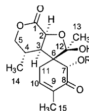
O -Acetylcyclocalopin A ( 2a ), R = Ac Cyclocalopin A ( 2b ), R = H
