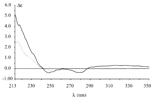
Figure 3. CD spectra of (+)-calopin ( 1b , solid line) and (+)-9-demethyl-7,8-dideoxycalopin ( 3 , dotted line) (CH 3 CN)
