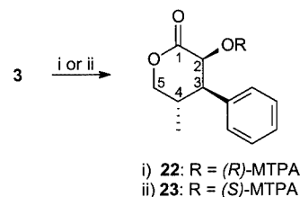
Scheme 5. Preparation of Mosher esters 22 and 23 ; reagents and conditions: i) ( S )-(+)-MTPA-Cl, NEt 3 , DMAP, CH 2 Cl 2 ; ii) ( R )-(-)-MTPA-Cl, NEt 3 , DMAP, CH 2 Cl 2 ; MTPA = \alpha -methoxy- \alpha -(trifluoromethyl)phenylacetic acid
