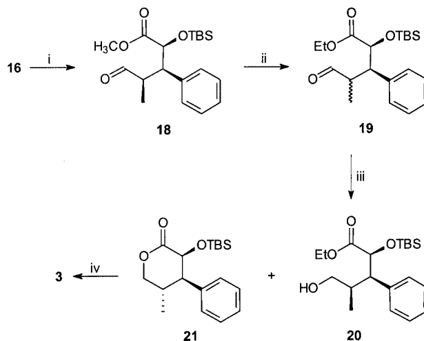
Scheme 4. Synthesis of \delta -valerolactone 3 ; reagents and conditions: i) (COCl) 2 , DMSO, NEt 3 , CH 2 Cl 2 , -78^\circ\text{C} ; ii) NaHCO 3 , EtOH, \Delta ; iii) NaBH 4 , MeOH, 0^\circ\text{C} , separation of 20 [34%, steps i)–iii)] and 21 [23%, steps i)–iii)]; iv) concd. HCl, THF, MeOH (96%)
