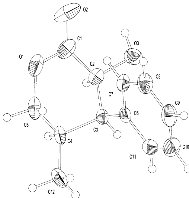
Figure 2. ORTEP plot derived from a single-crystal X-ray analysis of all- cis -valerolactone 11
