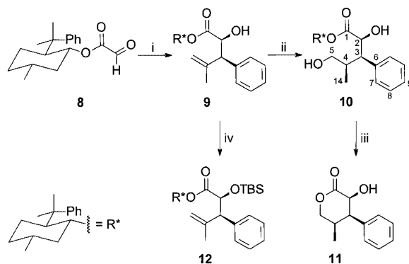
Scheme 2. Synthesis of all- cis \delta -valerolactone 11 ; reagents and conditions: i) \text{SnCl}_4 , 7 , \text{CH}_2\text{Cl}_2 , -78^\circ\text{C} \rightarrow -25^\circ\text{C} (81%); ii) 9-BBN or (+)- \text{Ipc}_2\text{BH} , THF, then NaOH, \text{H}_2\text{O}_2 , ultra sound (99%); iii) p\text{TsOH} , \text{CH}_2\text{Cl}_2 , 28^\circ\text{C} (63%); iv) TBSOTf, 2,6-lutidine, DMAP, \text{CH}_2\text{Cl}_2 (94%); \text{R}^* = (-) -8-phenylmenthyl, 9-BBN = 9-borabicyclo[3.3.1]nonane, \text{Ipc}_2\text{BH} = diisopinocampheylborane, TBS = tert -butyldimethylsilyl, DMAP = 4-(dimethylamino)pyridine
