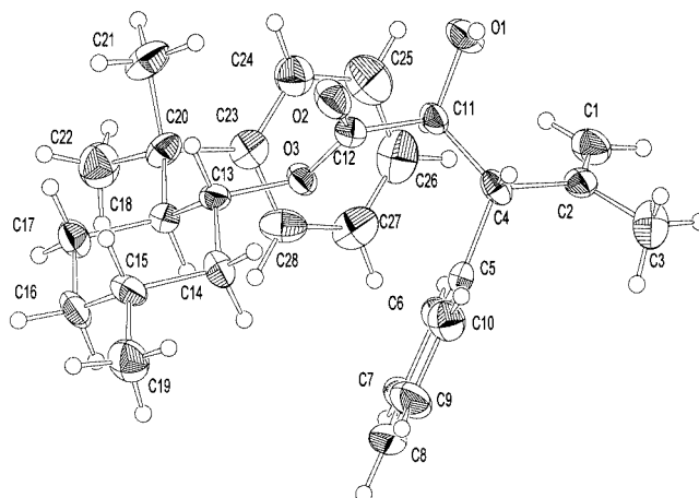
Figure 1. ORTEP plot derived from a single-crystal X-ray analysis of (–)-8-phenylmenthyl ester 9
